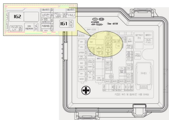
Fuel Cell Power Module Fuse Box
